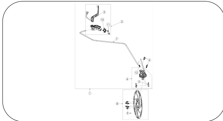
Picture 8 — REAR BRAKE
