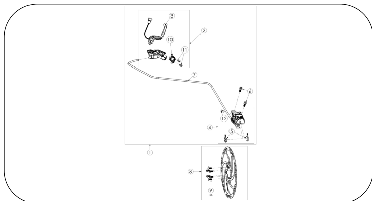
Picture 7 — FRONT BRAKE
