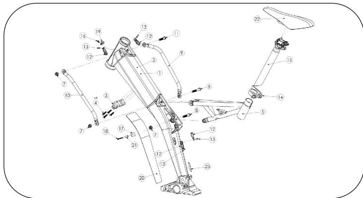
Picture 1 — CHASSIS WITH SEAT
